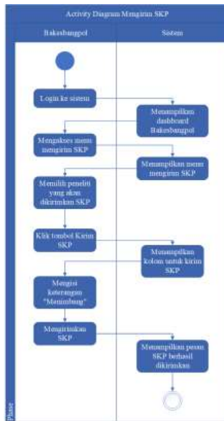
Gambar 4. Activity Diagram Mengirim SKP
